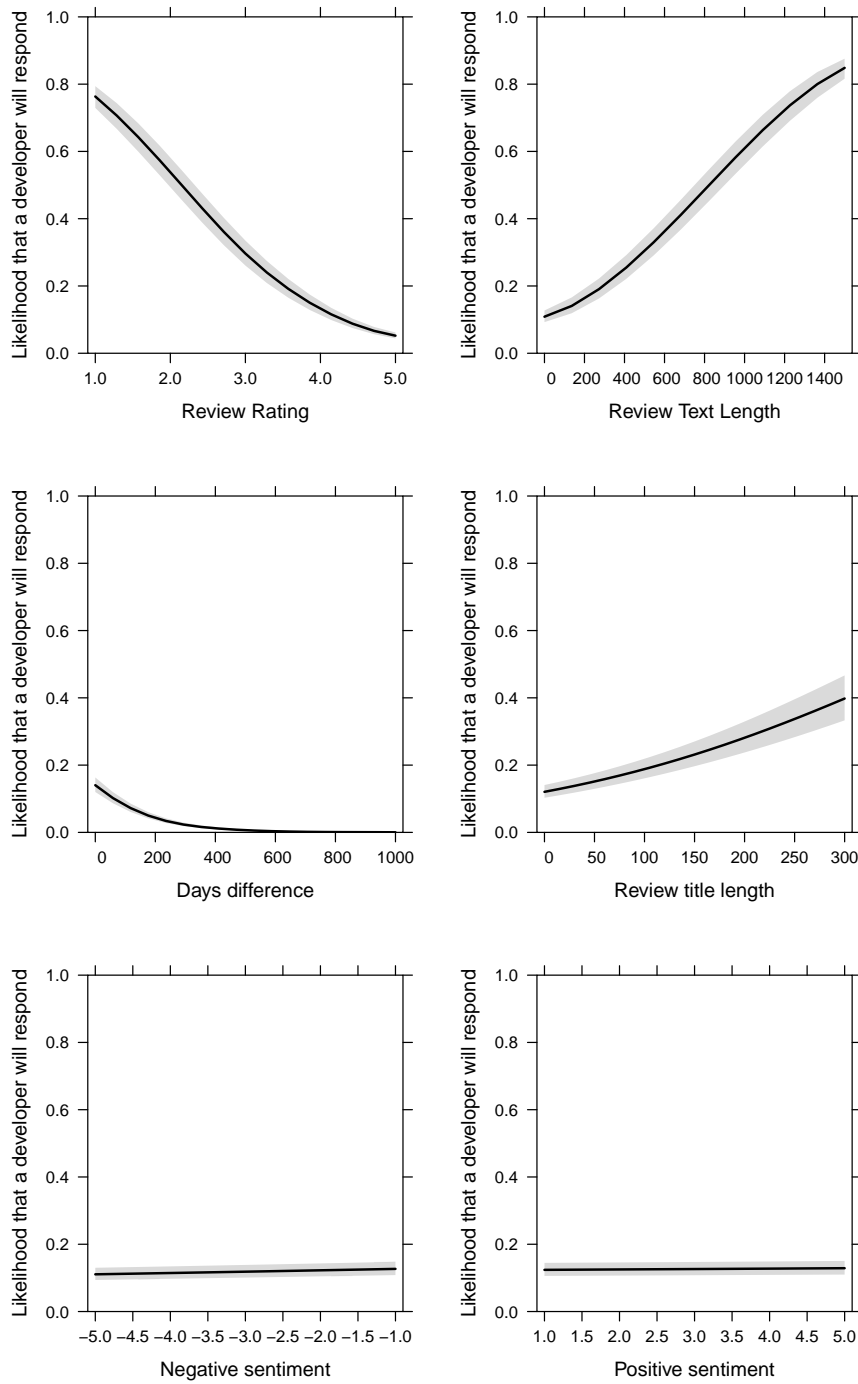
Fig. 6: The relationship between the review-level metrics and the likelihood that a developer will respond. The grey area represents the confidence interval. Note that these plots show the likelihood that a developer will respond for apps with responses to at least 5% of the reviews.
