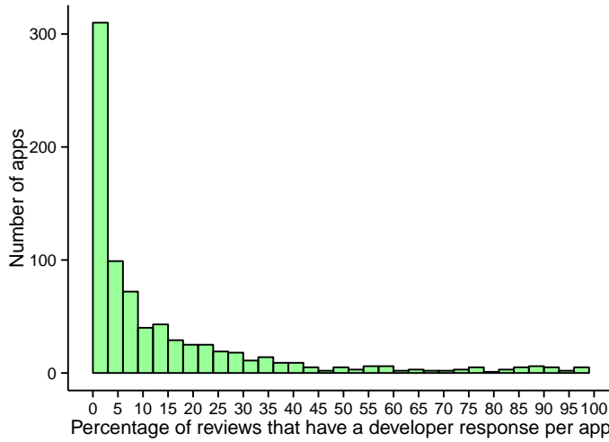
Fig. 3: The percentage of reviews to which a developer responded for each studied app. The figure displays only the 794 apps that have at least one review to which a developer responded.
