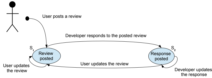
Fig. 1: User-developer dialogue in the Google Play Store
