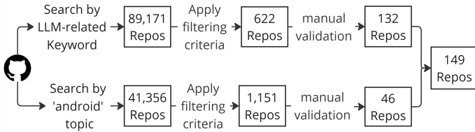
Fig. 1. Data collection overview.
