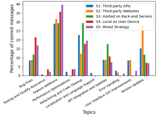
Fig. 15. The distribution of commit message topics per strategy.
